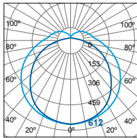
FOB80000v1-ds (17W)
