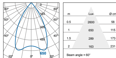
FDS72400v0-dm/db/sc-60°
