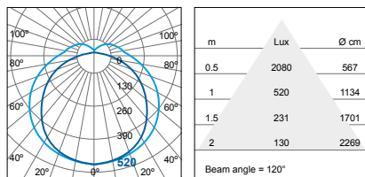
FOB80100v0-ds (17W)
