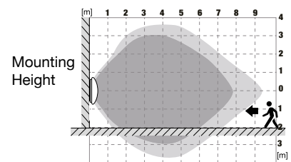
Wall Mounted
