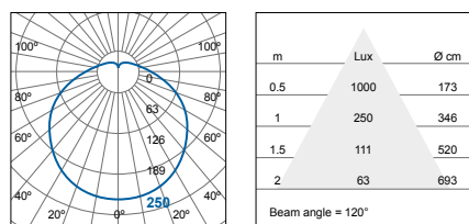
FCL72600v0-ds/sc FCL72600v0-ds/sc+LA10175 FCL72600v0-ds/sc+LA11149 FCL72600v0-ds/sc+LA10175+LA11149
