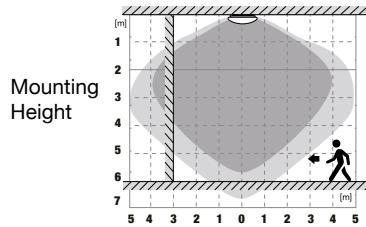
Ceiling Mounted
