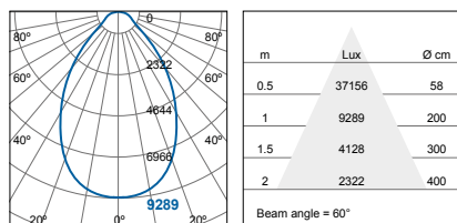
FFL74200v0-ds/sc+060D-90W FFL74200v0-ds+060D-90W
