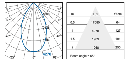
FLP70500v0-ds/sc (35W)
