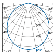
FCL73300v0-ds (6500K)
