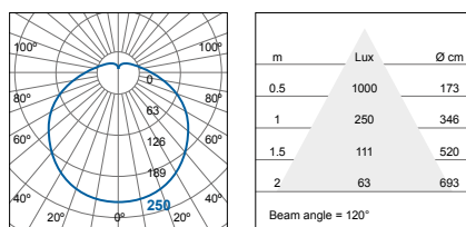
FCL72600v0-ds FCL72600v0-ds+LA10175 FCL72600v0-ds+LA11149 FCL72600v0-ds+LA10175+LA11149
